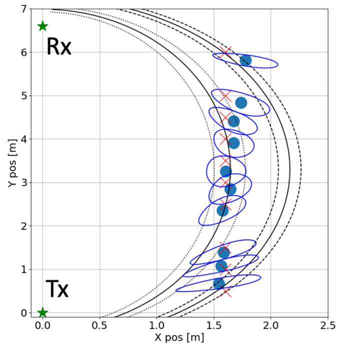
Figure 3. Bistatic ISAC for passive object detection with OFDM waveforms. The green stars represent the transmitter and receiver location. The red crosses show the ground-truth, the blue dots the estimates from angle measurements (included error ellipses), and the lines represent the distance measurements and their uncertainties.
