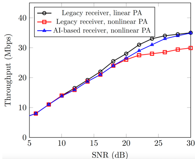
Figure 4 Performance of the AI-based receiver compared to the legacy receiver for PA post distortion compensation of DFT-s-OFDM signals.
