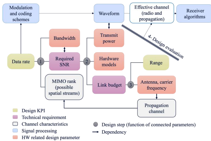
Figure 2 Radio design methodology for specifying radio design parameters to fulfil system requirements.
