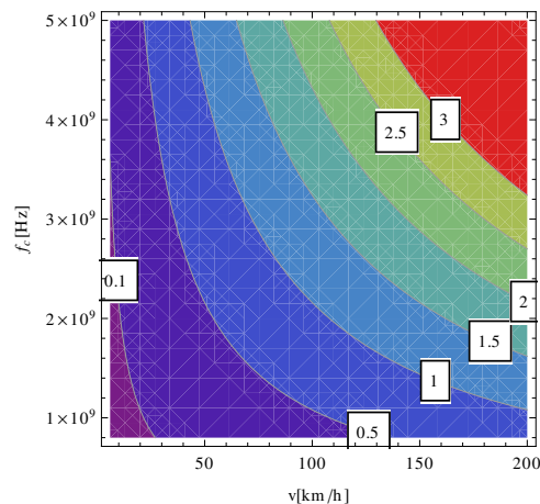
Fig. 2: Required prediction range expressed in carrier wavelengths corresponding to a prediction horizon of 5 ms, as a function of the vehicle velocity and the carrier frequency.
