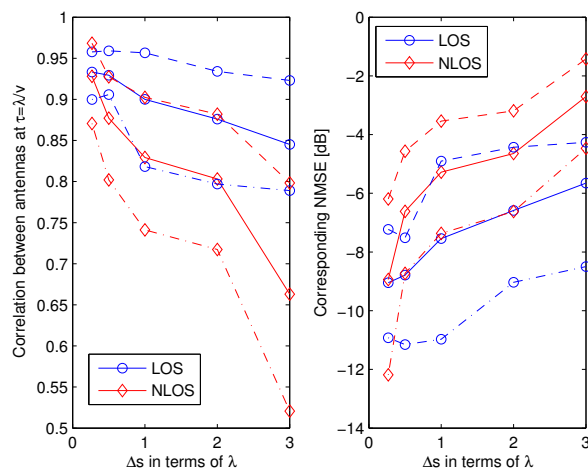
Fig. 7: Measured statistics for the peak correlation magnitude |c| (left) and the corresponding attainable NMSE 1 - |c|^2 (right). Solid: average over all subcarriers as a function of the distance between the antennas. Results for line-of-sight (rings, blue) and non-line-of-sight locations (diamonds, red). Dashed and dash-dotted lines represent the 95th and 5th percentiles, respectively.
